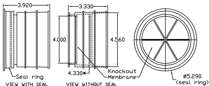
* I.D. reduces to accept SCH20 pipe. TE-4B OR TE-4BS 4" STEP-DOWN TERMINATOR (ACCEPTS SCH 40 OR SCH 20)
