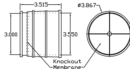
TE-3 3" TERMINATOR (ACCEPTS SCH 40 ONLY)
